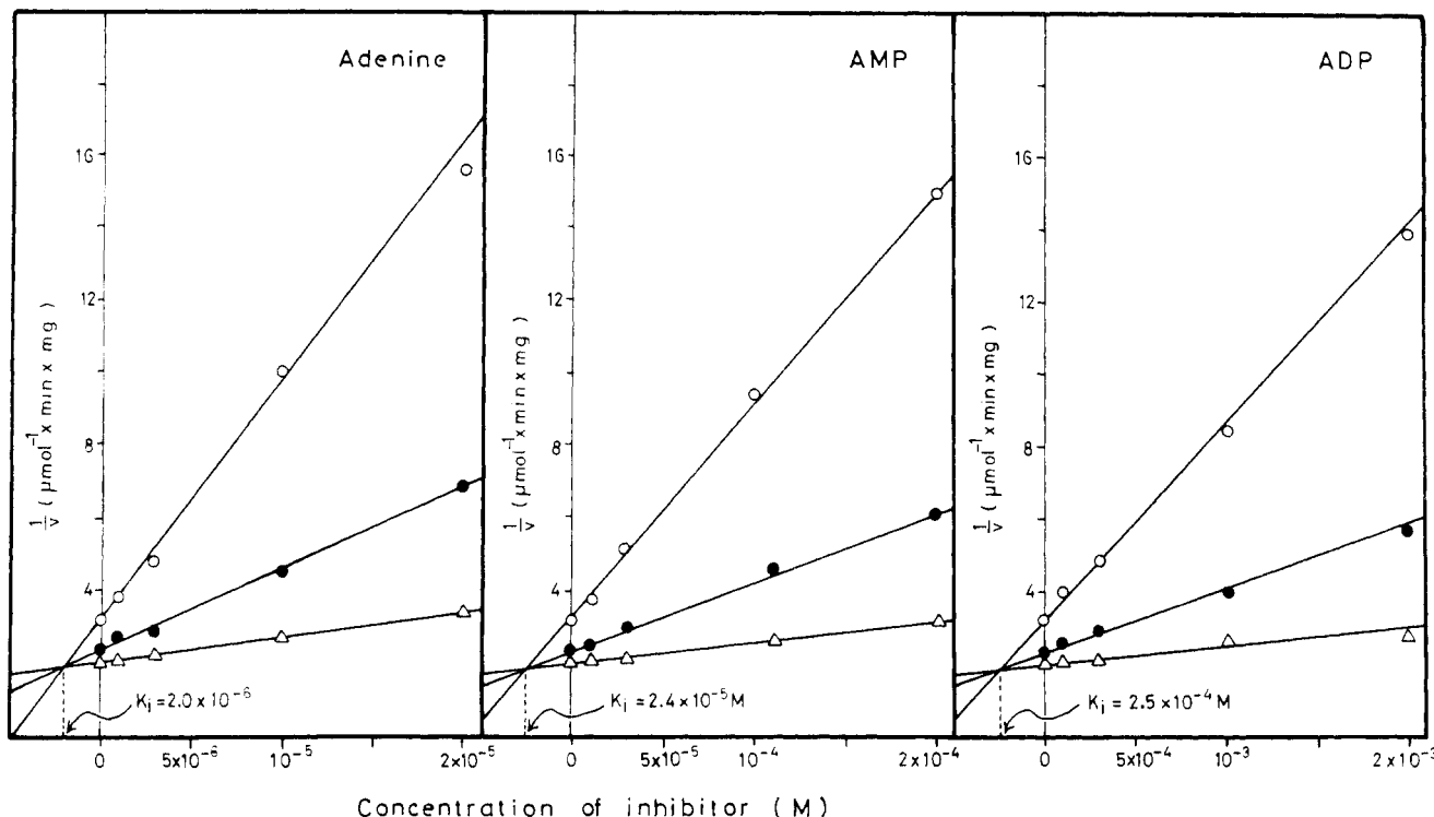
FIGURE 6: Inhibition of the hydrolysis of SAH by various concentrations of adenine, AMP, and ADP. The initial velocity ( v ) of the hydrolysis of 1 (○), 3 (●), and 10 \mu M (Δ) SAH was determined in the presence of adenine, AMP, and ADP at concentrations indicated on the figure. The data are plotted according to Dixon (1953).
