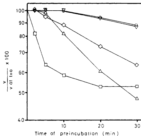
FIGURE 3: Effect of preincubation of the enzyme in the presence of adenine and adenine nucleotides on SAH synthase activity. S -Adenosylhomocysteinase ( 25\ \mu\text{g}/\text{mL} ) was preincubated for various periods of time in the presence of 25\ \mu\text{M} adenine ( \square ), 2\ \text{mM} AMP ( \nabla ), 2\ \text{mM} ADP ( \diamond ), 2\ \text{mM} ATP ( \Delta ), or no addition ( \circ ). The preincubation buffer was 15\ \text{mM} HEPES, pH 7.0, containing 0.25\% bovine serum albumin, 150\ \text{mM} KCl, 5\ \text{mM} magnesium acetate, and 2\ \text{mM} 2-mercaptoethanol, and the temperature was 37^\circ\text{C} . At times indicated on the figure, aliquots of 5\ \mu\text{L} were transferred to the assay mixture ( 300\ \mu\text{L} ) (see Materials and Methods) containing 5\ \mu\text{M} [ ^{14}\text{C} ]adenosine. The logarithm of the initial velocity is plotted against time of preincubation.
