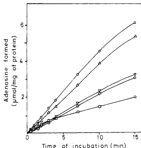
FIGURE 2: Time course of the hydrolysis of S -adenosylhomocysteine. [ ^{14}\text{C} ]Adenosylhomocysteine ( 5\ \mu\text{M} ) was incubated in the presence of enzyme ( 0.57\ \mu\text{g}/\text{mL} ) under the conditions described under Materials and Methods. The incubation mixture contained 10\ \mu\text{M} adenine ( \square ), 0.2\ \text{mM} AMP ( \nabla ), 2\ \text{mM} ADP ( \diamond ), 2\ \text{mM} ATP ( \Delta ), or no addition ( \circ ). The amount of adenosine formed is plotted against time of incubation.
