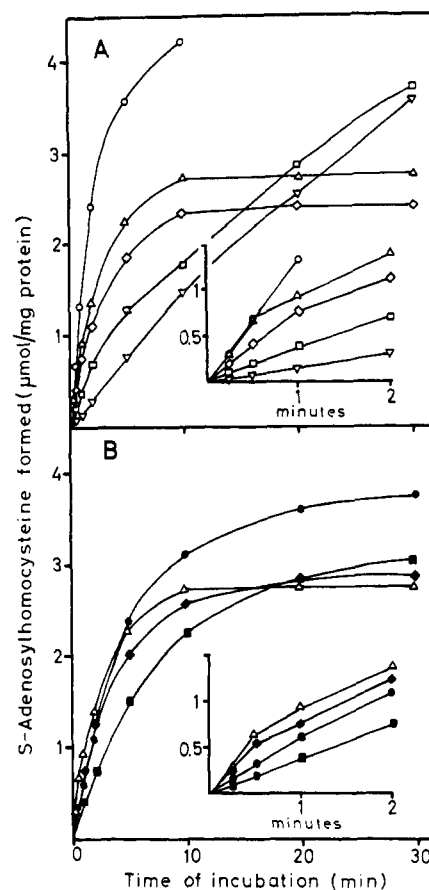
FIGURE 1: Time course of the synthesis of S -adenosylhomocysteine. (A) [ 14 C]Adenosine (1 μM) was incubated in the presence of homocysteine and enzyme (0.23 μg/mL) under the conditions described under Materials and Methods. The incubation mixture was supplemented with 30 μM adenosine (□), 1 mM AMP (▽), 1 mM ADP (◇), 2.5 mM ATP (Δ), or no addition (○). The amount of SAH formed is plotted vs. time of incubation. The inset shows the same data at a short time of incubation. (B) The formation of SAH was determined in the presence of 2.5 mM ATP as described above except that the incubation buffer contained no Mg and KCl (●), 5 mM Mg (◆), 5 mM Mg and 150 mM KCl (Δ), or 5 mM Mg, 150 mM KCl, and 5 μM SAH (■). The data are plotted as described in (A).
